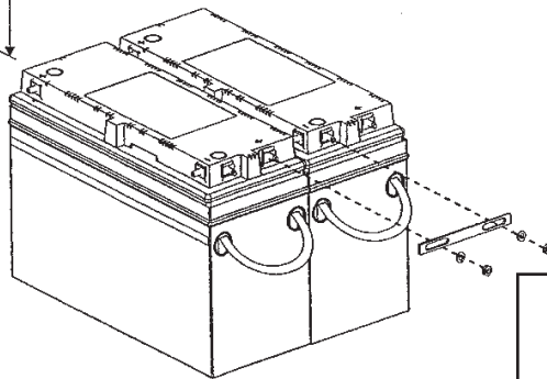
Figure 2: 12AVR-125L Bus Bar
