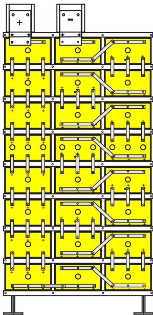
Front view 24 x 2CMT 6 post cells
