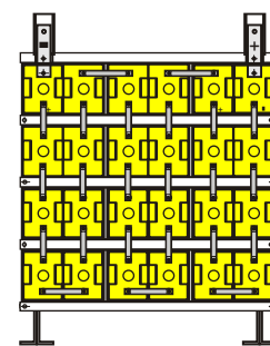
Front view 24 x 2CMT 2 post cells
