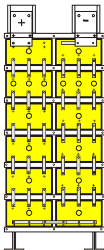
Front view 12 x 2CMT 6 post cells
