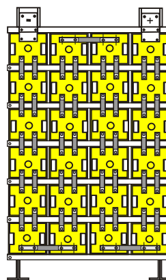
Front view 24 x 2CMT 4 post cells
